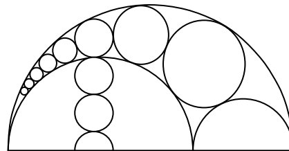
FIGURE 3.2: Classical Pappus’ Arbelos Theorem: the base is divided randomly, yet every circle in the chain is an even multiple of its radius above the axis.
