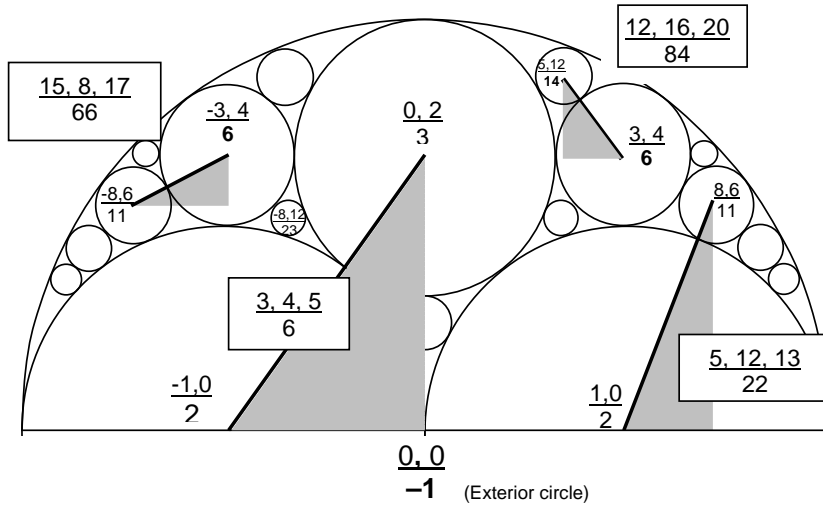
FIGURE 4.1: Pythagorean triples in the Apollonian Window
