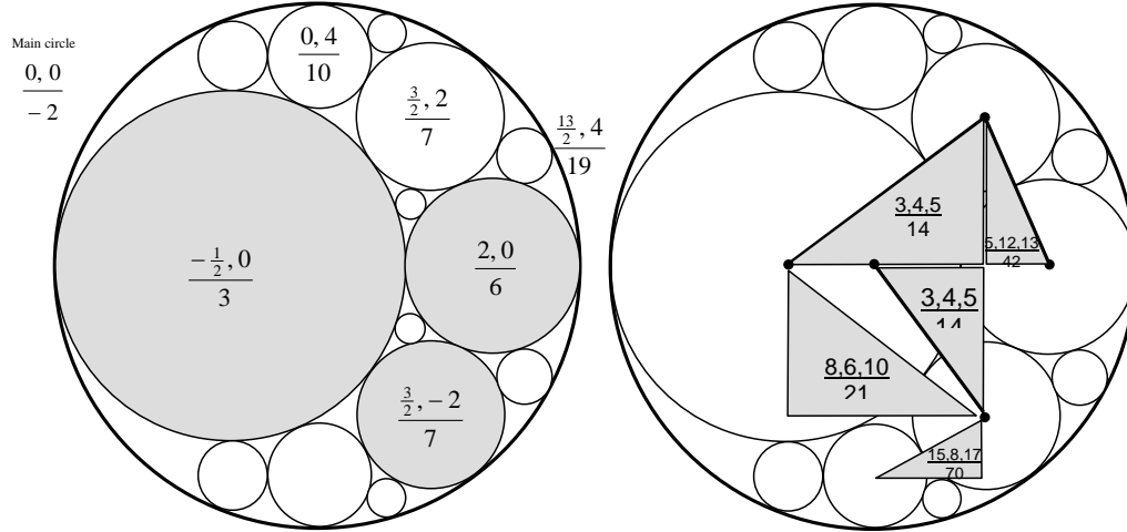
FIGURE 6.1: Arrangement (b_0, b_1, b_2, b_3) = (-2, 3, 6, 7) or (B, \mu, k, n) = (2, 4, 4, 5) . Left side shows symbols of the principal and other circles, right side shows Pythagorean triples.
