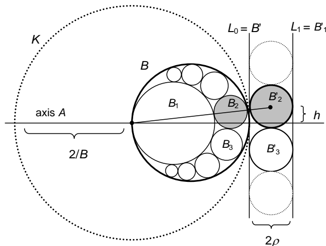
FIGURE 2.3: The method of inversion.
