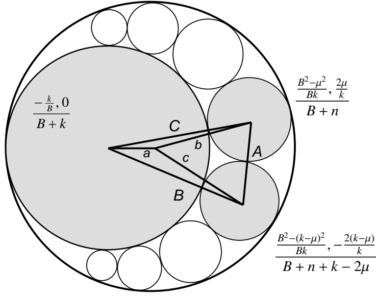
FIGURE 4.2: Labels of circles in the Apollonian packing [B, \mu, n, k]
