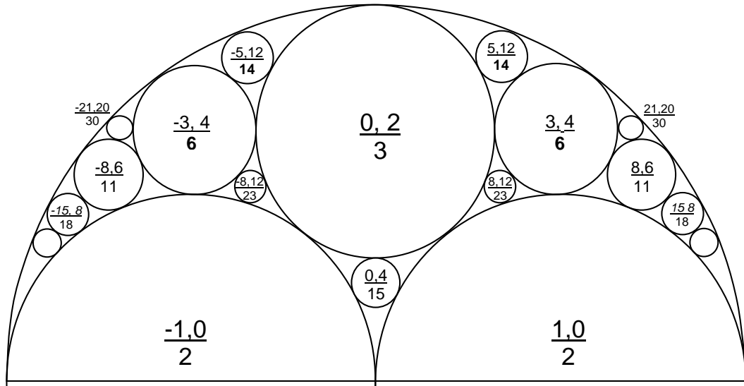
FIGURE 3.1: Apollonian Window with labels.
