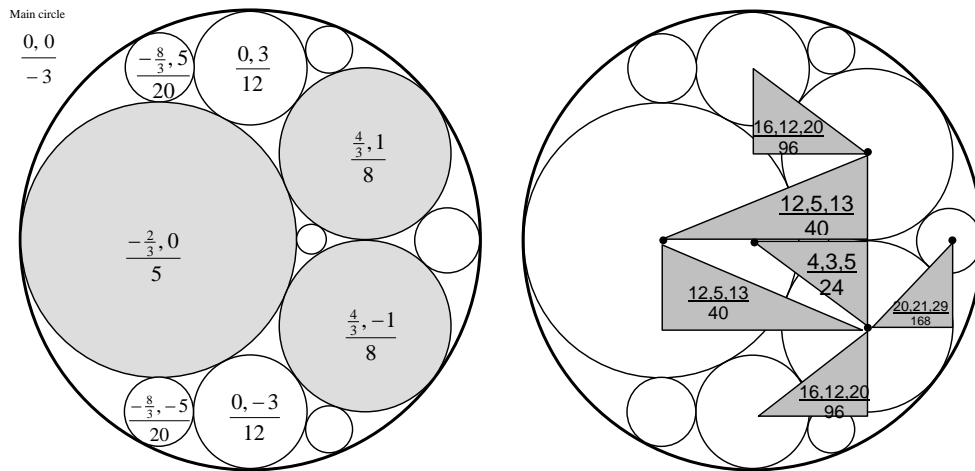
FIGURE 6.2: Arrangement (b_0, b_1, b_2, b_3) = (-3, 5, 8, 8) or (B, \mu, k, n) = (3, 4, 5, 5) . Both symbols (left) and Pythagorean triples (right). The triangles are reported with absolute values of sides.
