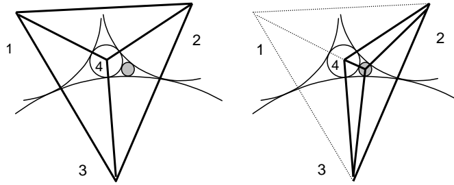
FIGURE 5.1: (a) A frame (b) and an adjacent frame. Circle 4' is shaded.
