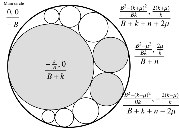
FIGURE 3.3: Labels of circles in the Apollonian packing [B, \mu, n, k]
