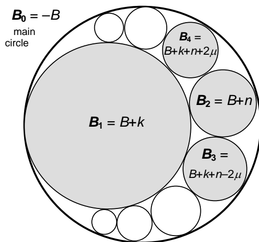
FIGURE 2.1: An Apollonian gasket and its four greatest circles (smallest curvatures)
