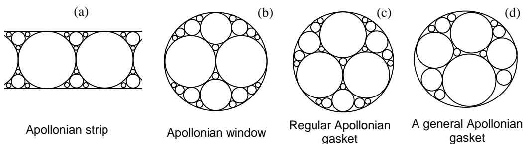
FIGURE 1.1: Various Apollonian disk packings
