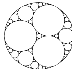
FIG. 3. The extended set S^* .
