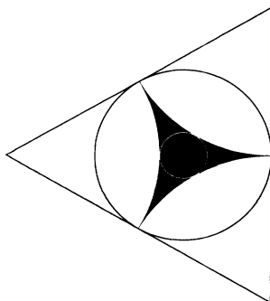
FIG. 2. The inscribed circle, the subset, the dual circle, and the triangle corresponding to one and the same word.
