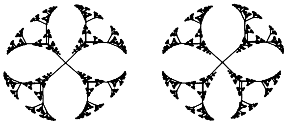
FIG. 5. The Apollonian tree in the Poincaré sphere representation (stereo picture).
