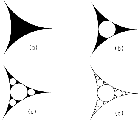
FIG. 1. Some low-order approximations to the Apollonian set \mathcal{S} : (a) \mathcal{S}^{(0)} , (b) \mathcal{S}^{(1)} , (c) \mathcal{S}^{(2)} , and (d) \mathcal{S} itself.
