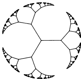
FIG. 4. The Farey tree (\infty, 3) in the Poincaré circle. It does a Farey organization of the boundary r = 1 .
